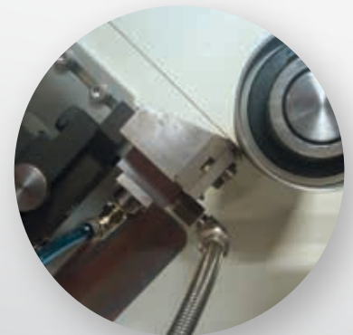
Micro-Adjust Rigid Bracket Assembly for Precision Coating
